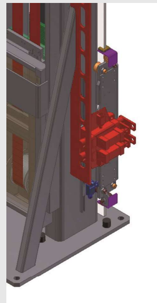
ABL Absteckung 2-Bolzen-Lochleiste ABL safety stacking unit 2-bolt-hole-strip
